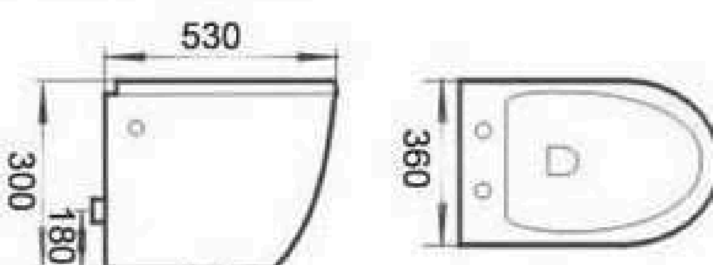
LE8505 Collision type flush Wall-hung Closet Size: 530x360x300mm P-trap: 180mm
