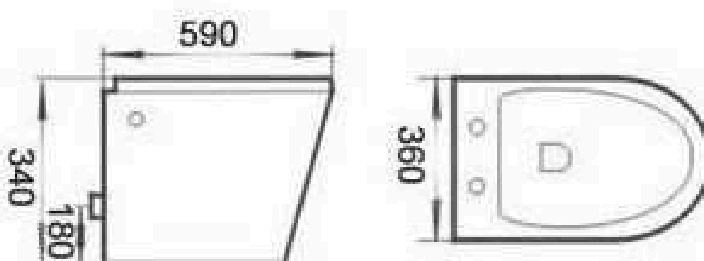
LE8502 Eddy double hole Wall-hung Closet Size: 590x360x340mm P-trap: 180mm
