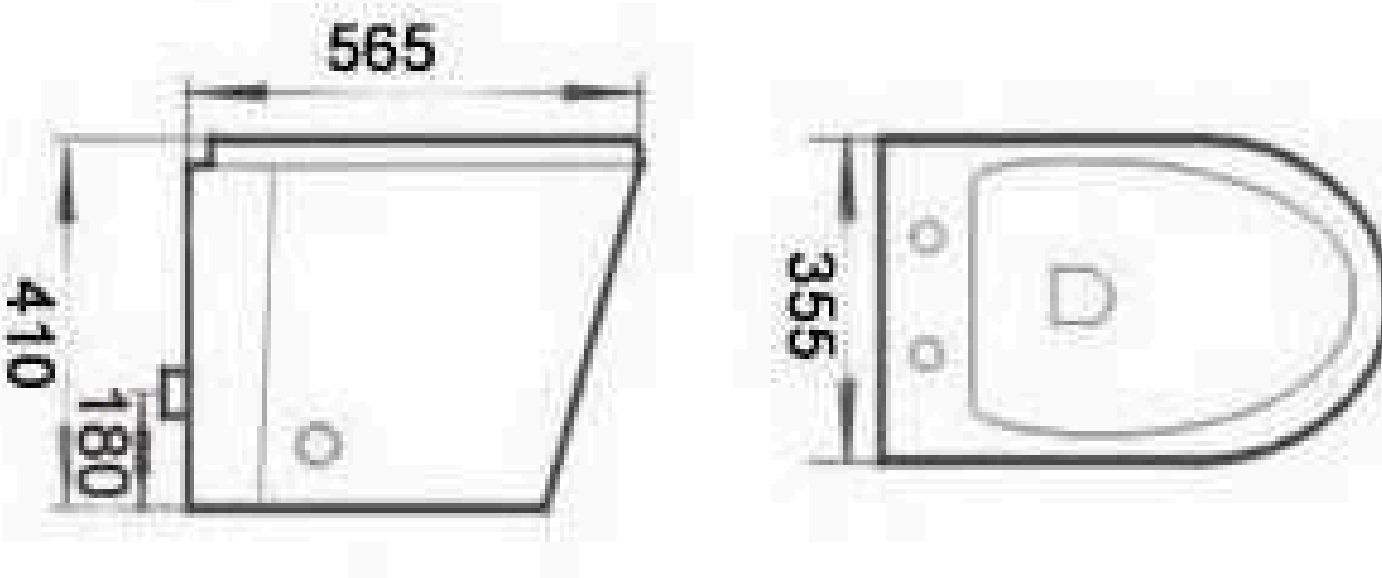
LE8511 Washdown Wall-hung Closet Size: 565x355x410mm P-trap: 180mm
