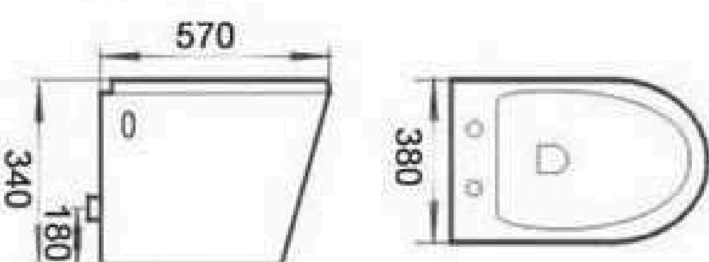
LE8506 Washdown Wall-hung Closet Size: 570x380x340mm P-trap: 180mm
