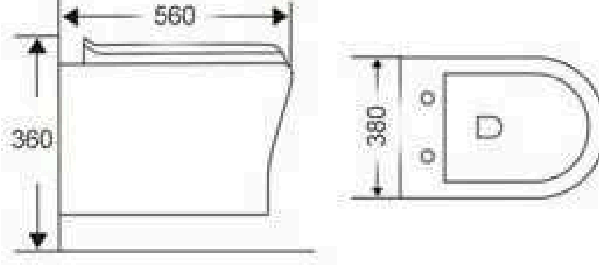
LE8517 Washdown Wall-hung Closet Size: 560x380x360mm P-trap: 180mm
