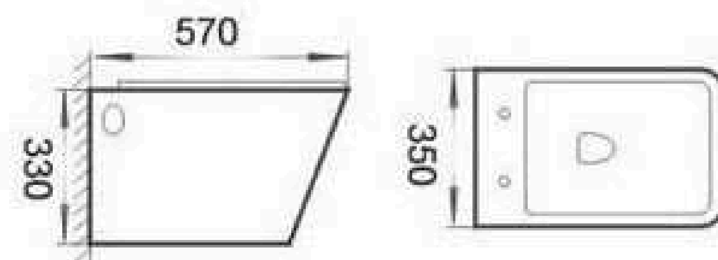
LE8507 Washdown Wall-hung Closet Size: 570x350x330mm P-trap: 180mm
