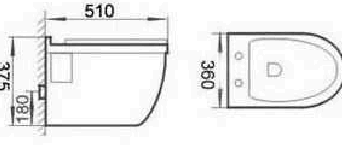
LE8516 Washdown Wall-hung Closet Size: 510x360x375mm P-trap: 180mm
