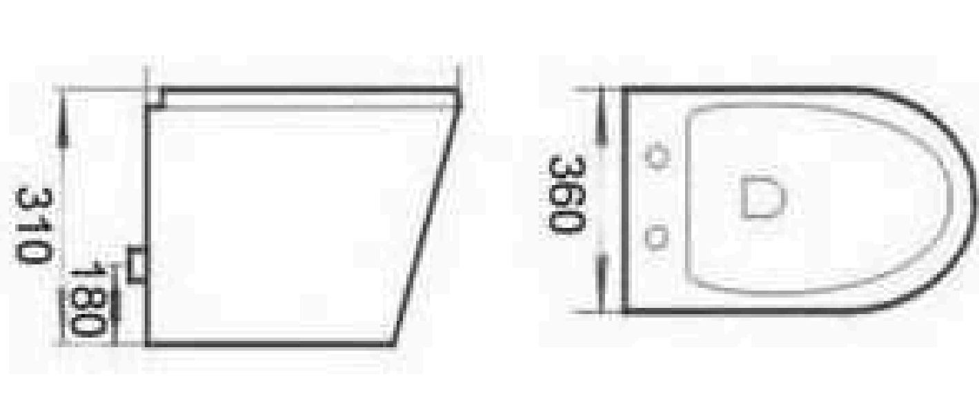
LE8520 Collision type flush Wall-hung Closet Size: 520x360x310mm P-trap: 180mm
