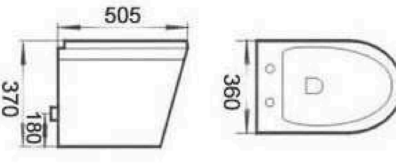
LE8514 Collision type flush Wall-hung Closet Size: 505x360x370mm P-trap: 180mm
