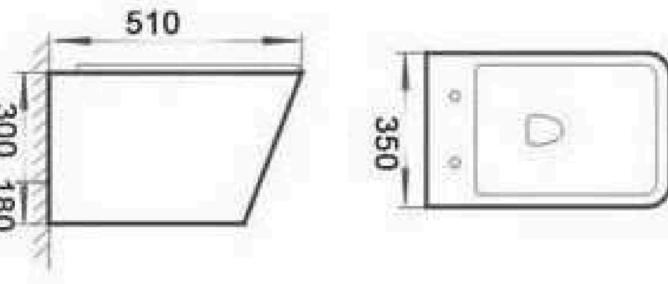
LE8513 Washdown Wall-hung Closet Size: 510x350x300mm P-trap: 180mm
