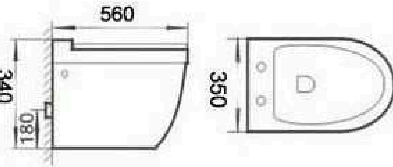
LE8510 Washdown Wall-hung Closet Size: 560x350x340mm P-trap: 180mm
