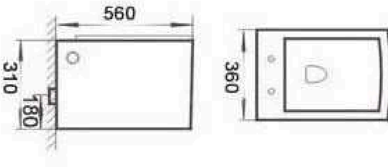
LE8512 Washdown Wall-hung Closet Size: 560x360x310mm P-trap: 180mm
