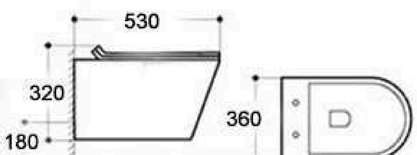
LE8508 Washdown Wall-hung Closet Size: 530x360x320mm P-trap: 180mm
