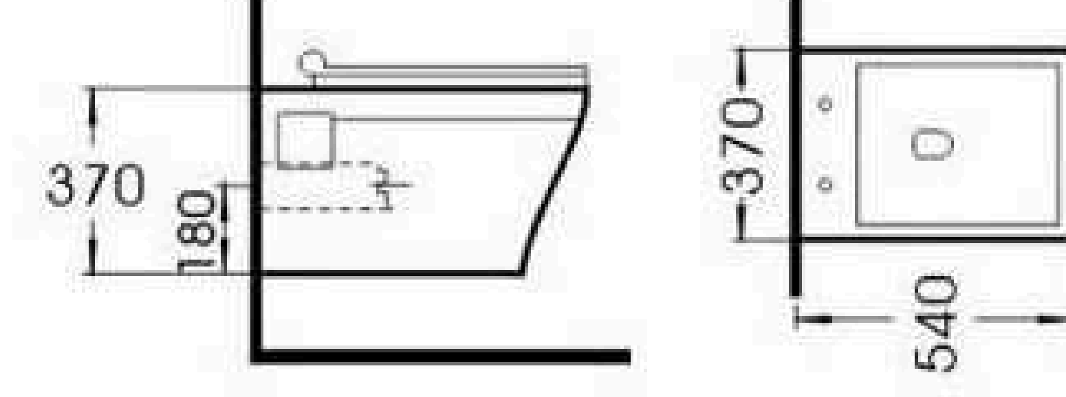
LE8519 Rimless flushing Wall-hung Closet Size: 540x370x370mm P-trap: 180mm
