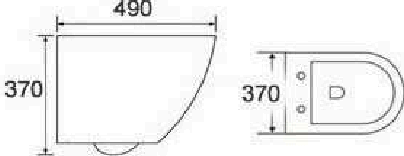
LE8501 Collision type flush Wall-hung Closet Size: 490x370x370mm P-trap: 180mm
