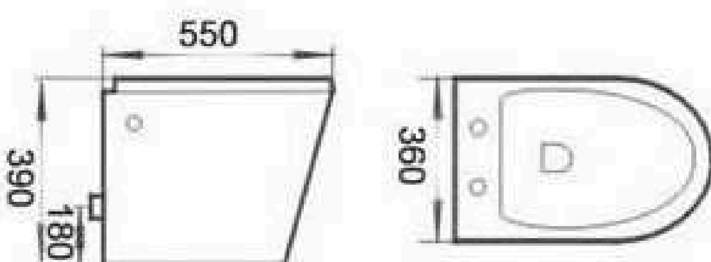
LE8503 Washdown Wall-hung Closet Size: 550x360x390mm P-trap: 180mm
