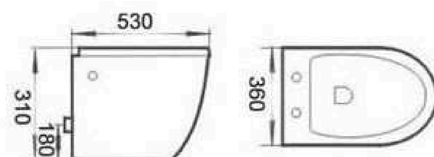
LE8504 Eddy double hole Wall-hung Closet Size: 530x360x310mm P-trap: 180mm
