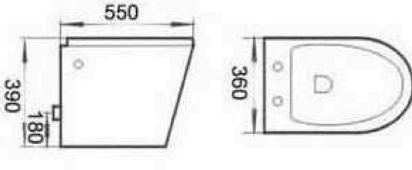
LE8503MW Washdown Wall-hung Closet Size: 550x360x390mm P-trap: 180mm
