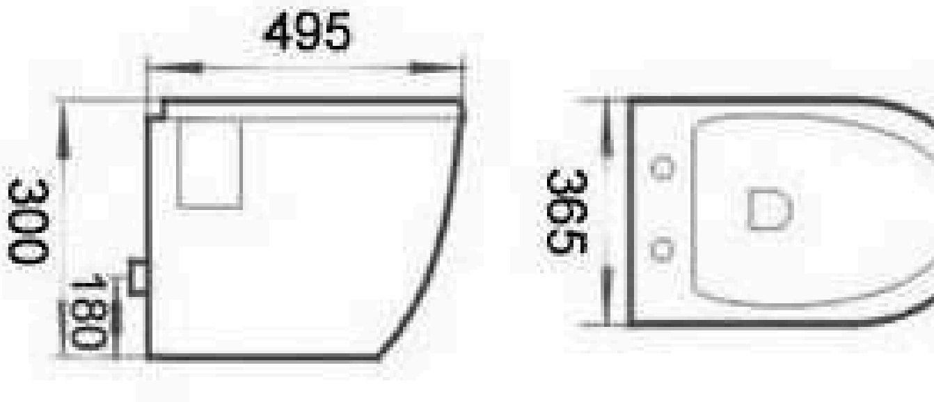
LE8518 Rimless Wall-hung Closet Size: 495x365x300mm P-trap: 180mm
