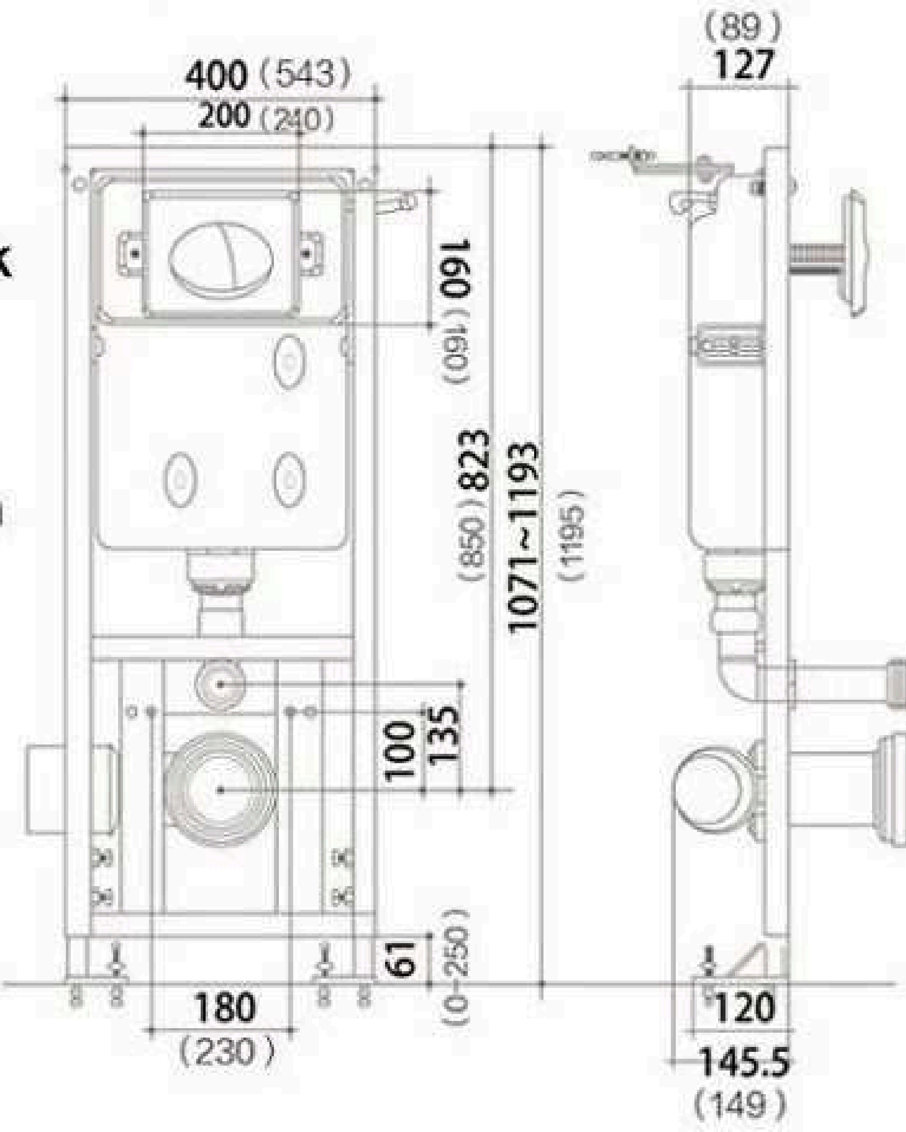
LE1101 Size: 543x89x1195mm LE1102 Size: 400x127x1071-1193mm
