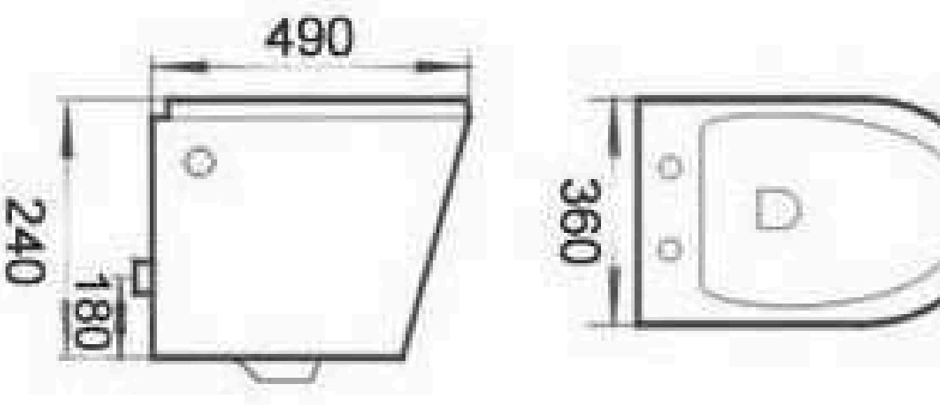
LE8515 Collision type flush Wall-hung Closet Size: 490x360x240mm P-trap: 180mm
