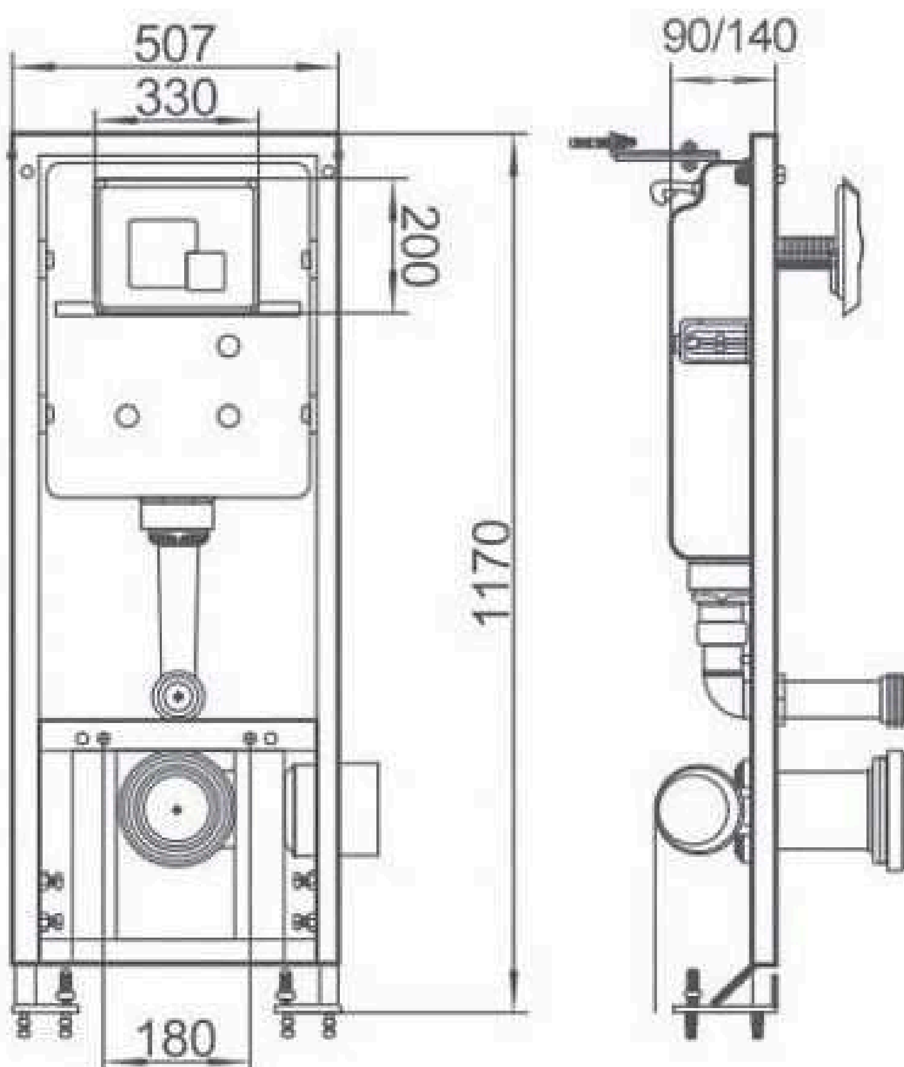
LE1103 Size: 507x90x1170mm LE1104 Size: 507x140x1070mm
