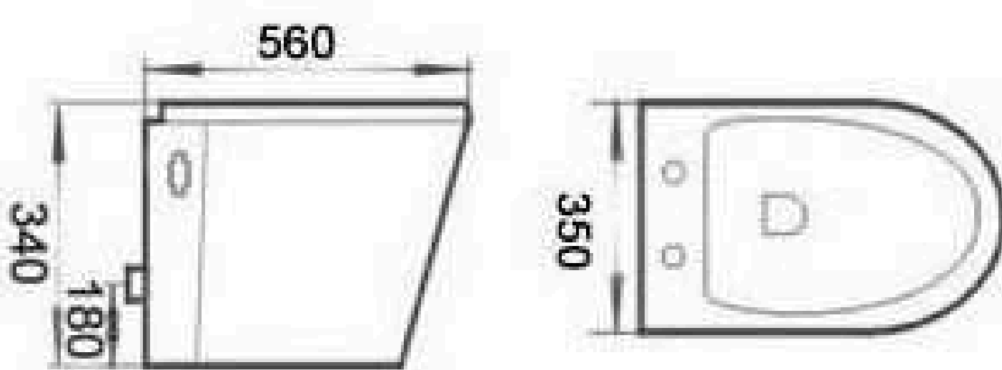
LE8509 Washdown Wall-hung Closet Size: 560x350x340mm P-trap: 180mm
