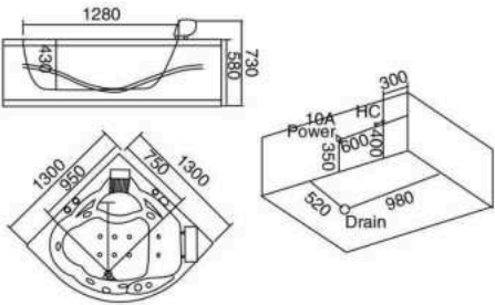
Model:CA-5007 Size:1300x1300x580mm
