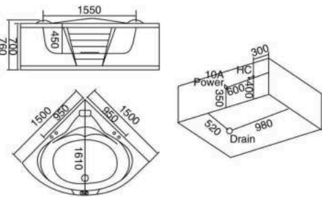
Model:CA-5008 Size:1500x1500x700mm
